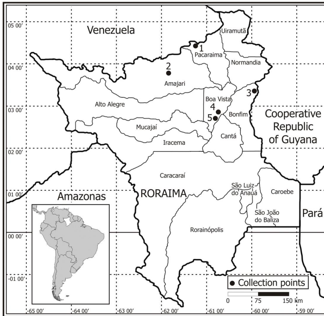
Figure 1. Map of the state of Roraima showing the locations of the McPhail* traps used for chrysopid collection in the four studied municipalities.
